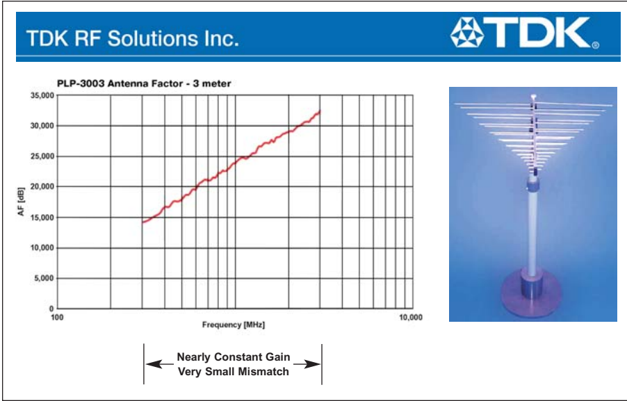
Figure 1 · Antenna Factor (AF) vs. frequency of a typical measurement antenna.
